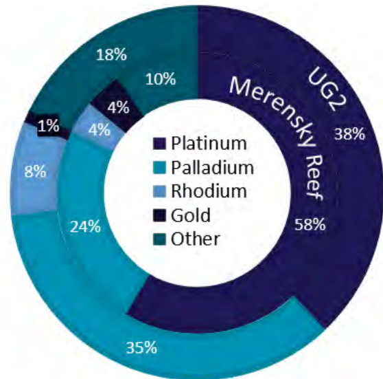
Figure 2: Merensky and UG2 Reef Prill Split
