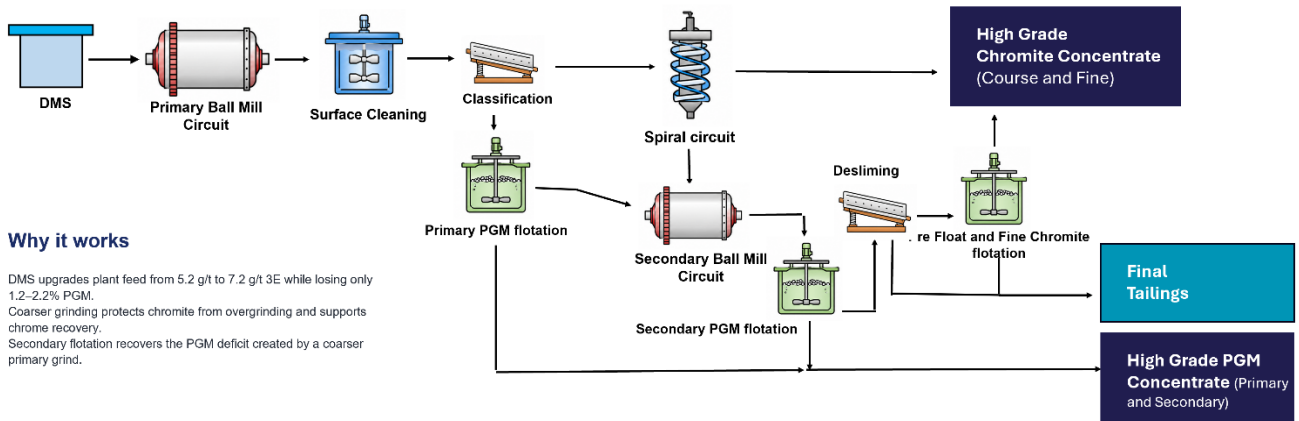
Figure 5: Proposed conventional processing route with DMS pre-concentration, coarser grinding, interstage chrome recovery and primary/secondary PGM flotation.
