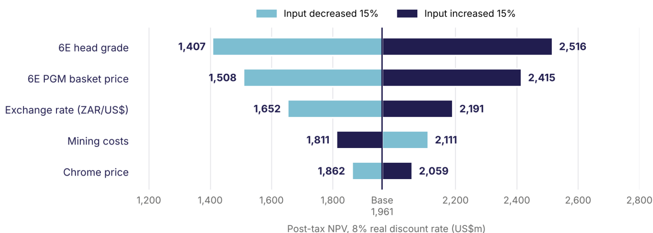
Figure 4: Sensitivity of post-tax NPV (US$m, 8% real discount rate) to ±15% changes in key inputs, holding all other inputs constant. A higher ZAR/US$ rate represents a weaker rand.
