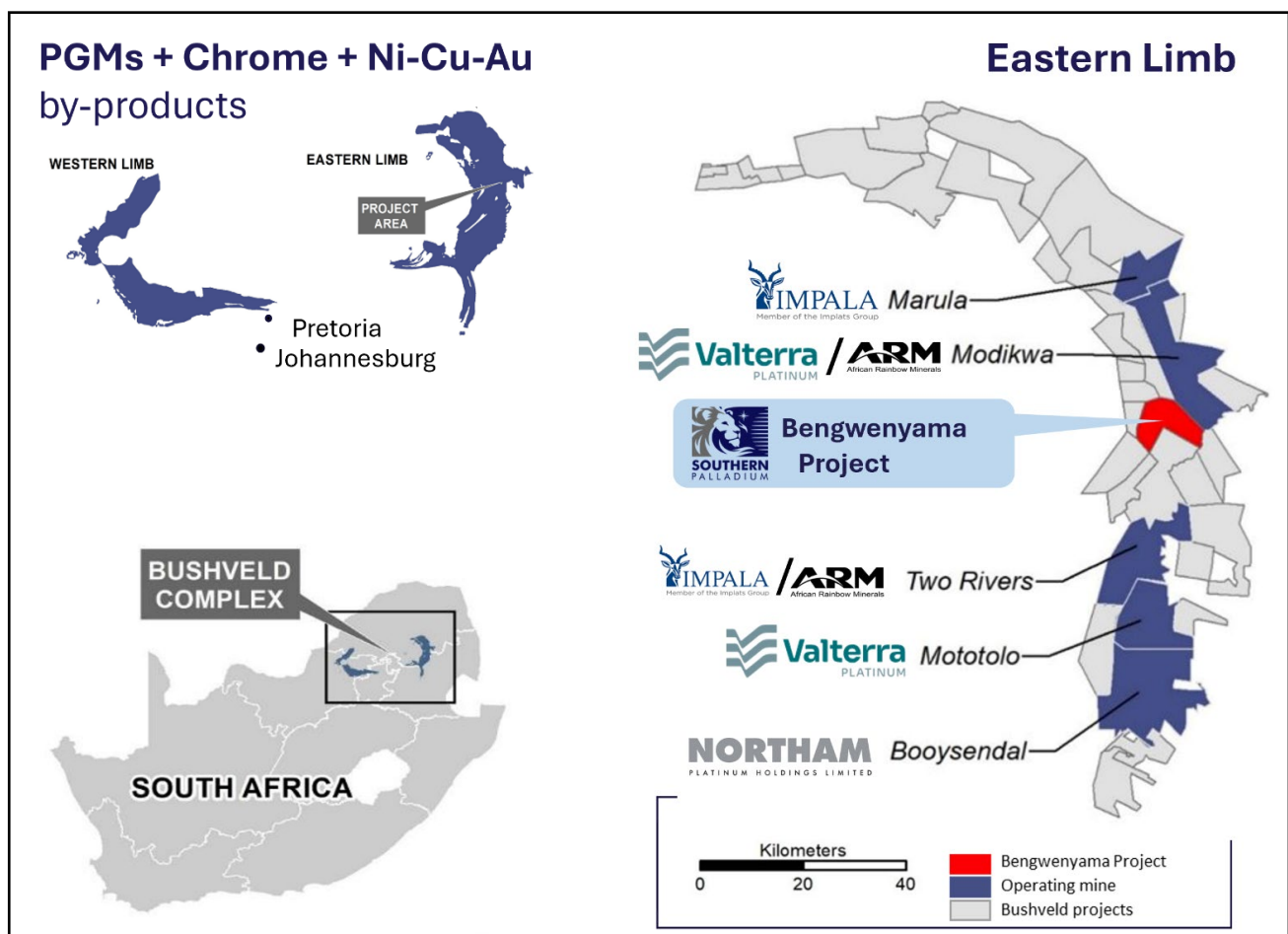
Figure 1: Bengwenyama's location on the Eastern Limb of the Bushveld Complex relative to neighbouring PGM operations.
